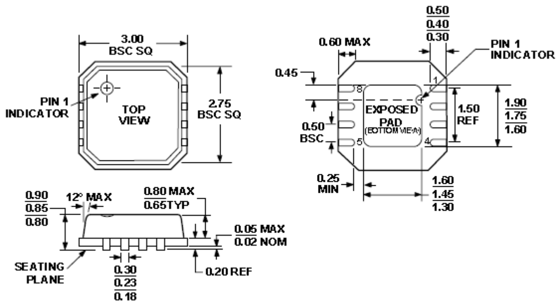
8-Lead Lead Frame Chip Scale Package [LFCSP]
