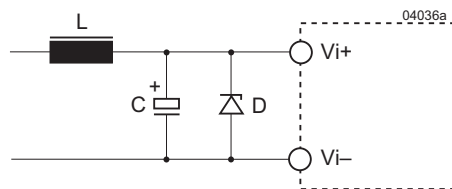
Fig. 6 Example for external circuitry to achieve better transient immunity. The diode D is only necessary for 20IMX15 models.
